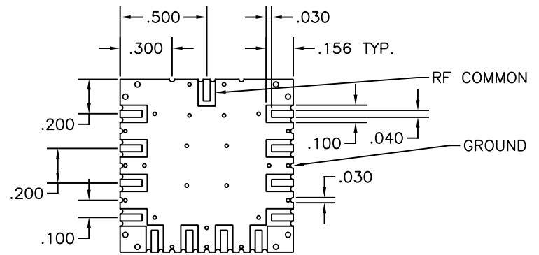
BOTTOM VIEW
